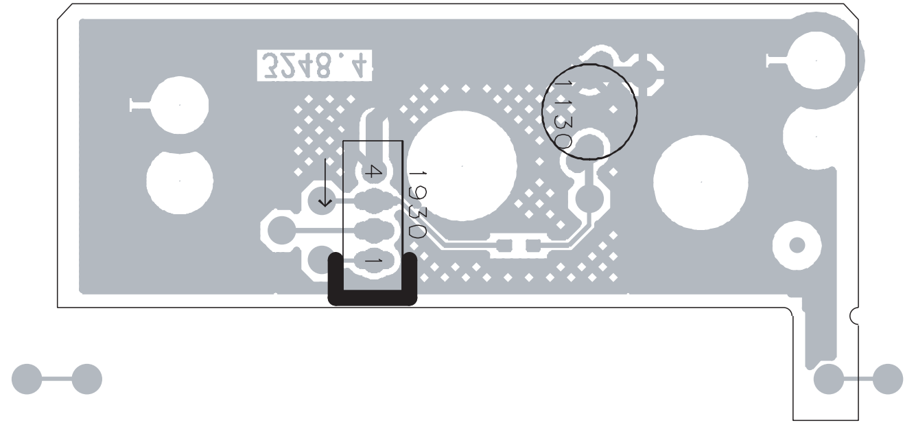
StbyBd_3139_243_32484_TopView.pdf 2005-08-22
